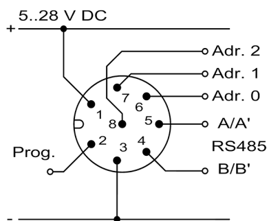
Fig. 14: RS485 connection
