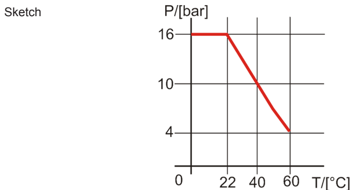
Fig. 11: PVC-U diagram
