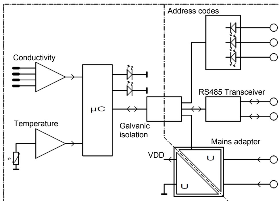
Fig. 4: Block diagram
